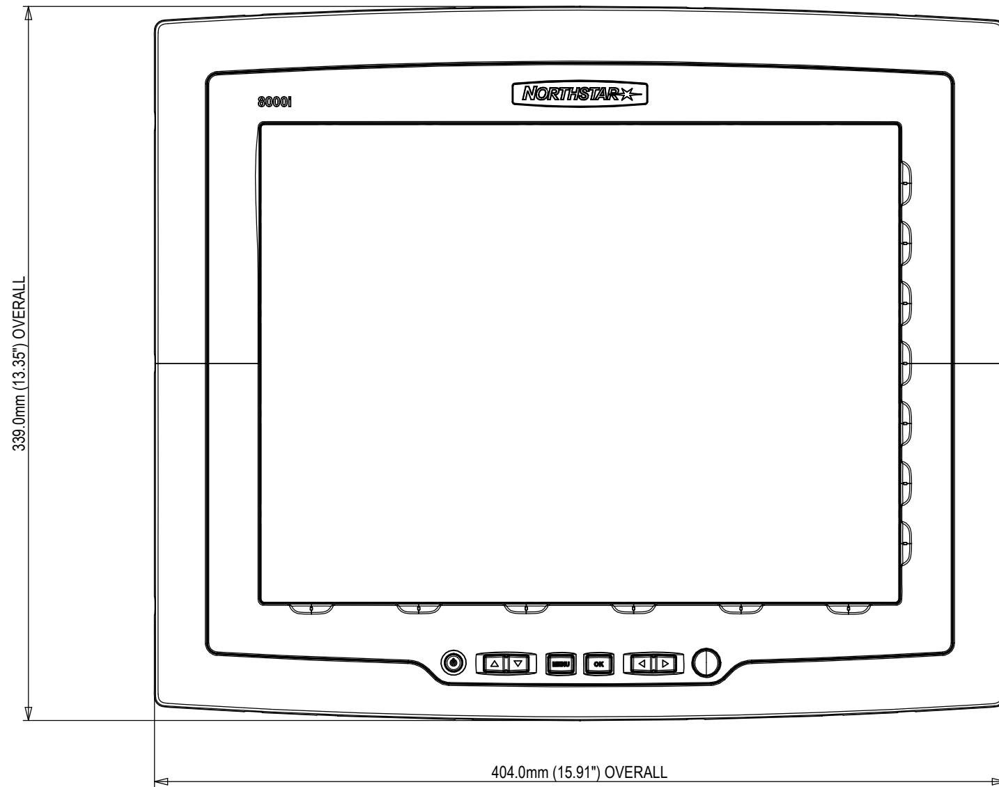
Northstar 8000i 15" Monitor Overall Sizes
